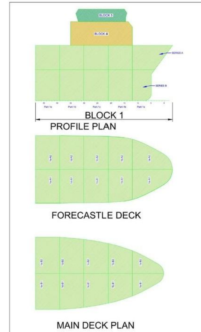
Profile and Plan views of the Block – 1 section is shown below,
